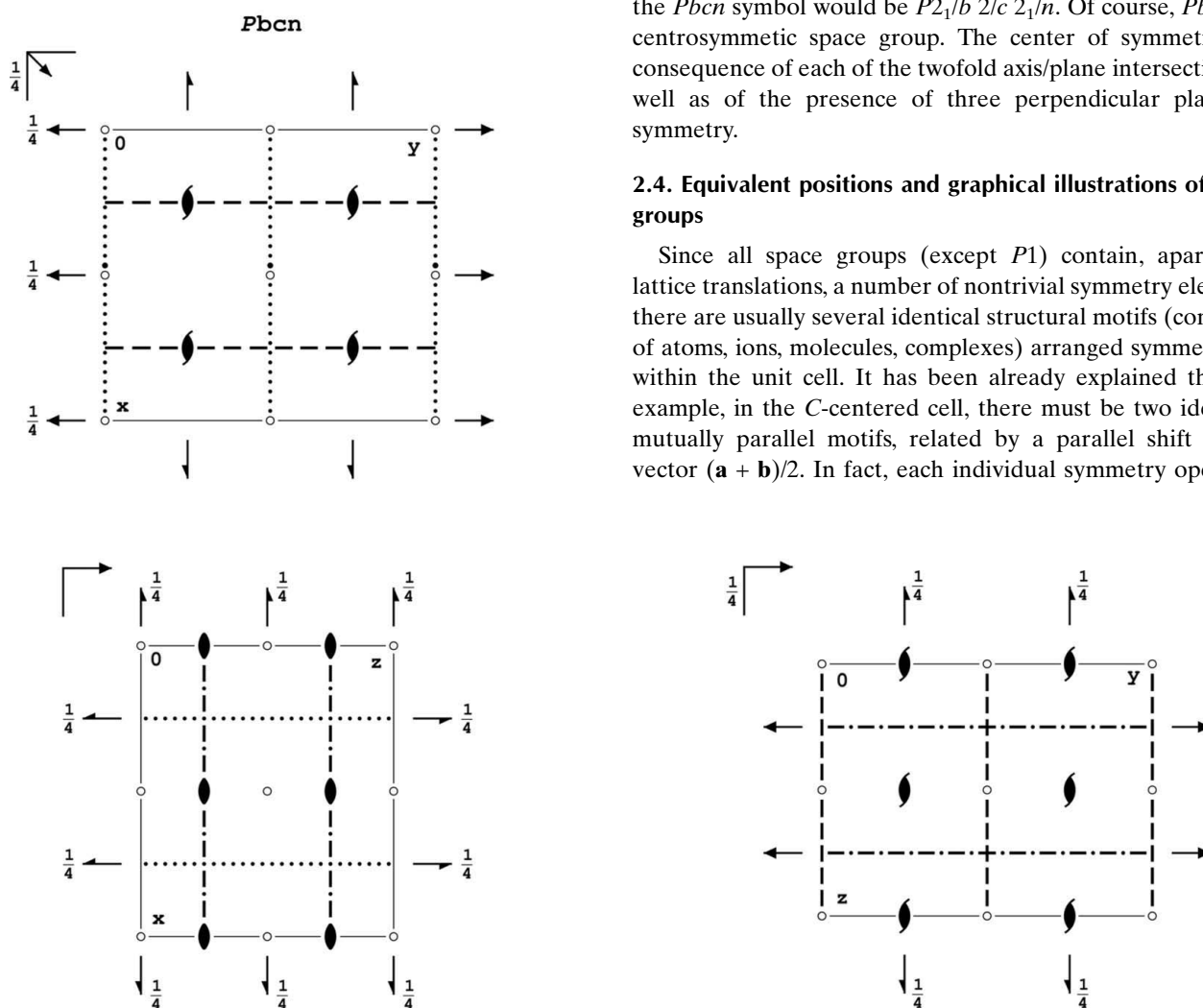
Figure 14 Symmetry diagrams of the orthorhombic space group Pbcn , shown in projections along z (top), y (lower left) and x (lower right).
