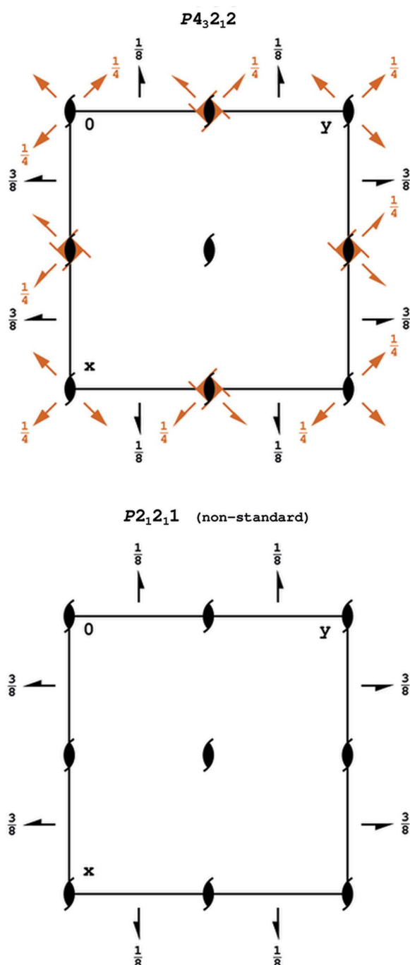
Figure 26 Reduction of P4_32_12 to its subgroup P2_12_12_1 , by the removal of the symmetry elements shown in brown.
