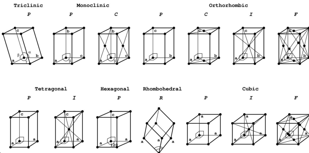
Figure 8 The 14 Bravais lattices.
