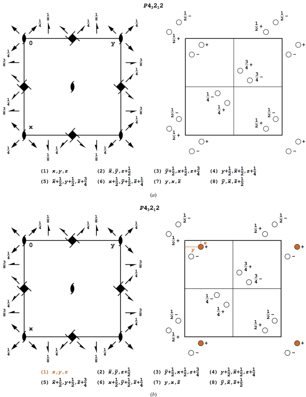
Figure 15 (a) A diagram with symmetry elements (left) and with equivalent points (represented by circles) in general positions (right), together with the fractional coordinates (numbered) of those equivalent positions (bottom list) presented for the space group P4_32_12 in the style of ITA. The numbers near the equivalent points refer to their elevation above (or below) the ab base of the unit cell (for example, \frac{1}{2}- stands for \frac{1}{2} - z ). (b) The same diagrams as in (a) but with the principal point with coordinates (x, y, z) highlighted in brown. Also highlighted are its x - and y -translation equivalents. Coordinates like these (brown), generated by pure lattice translations, are not listed in ITA.
