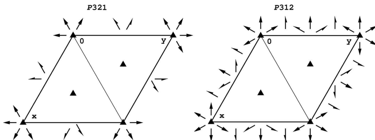
Figure 13 Diagrams of symmetry operations for two trigonal space groups: (left) P321 and (right) P312 .
